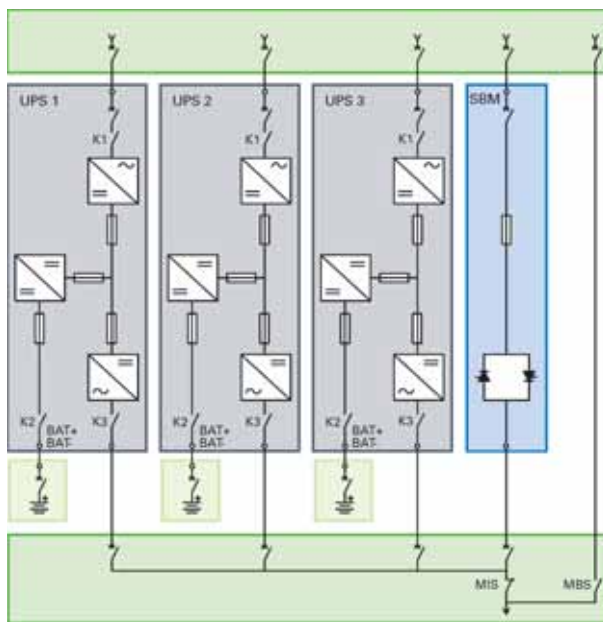
Parallel system with a centralised bypass
