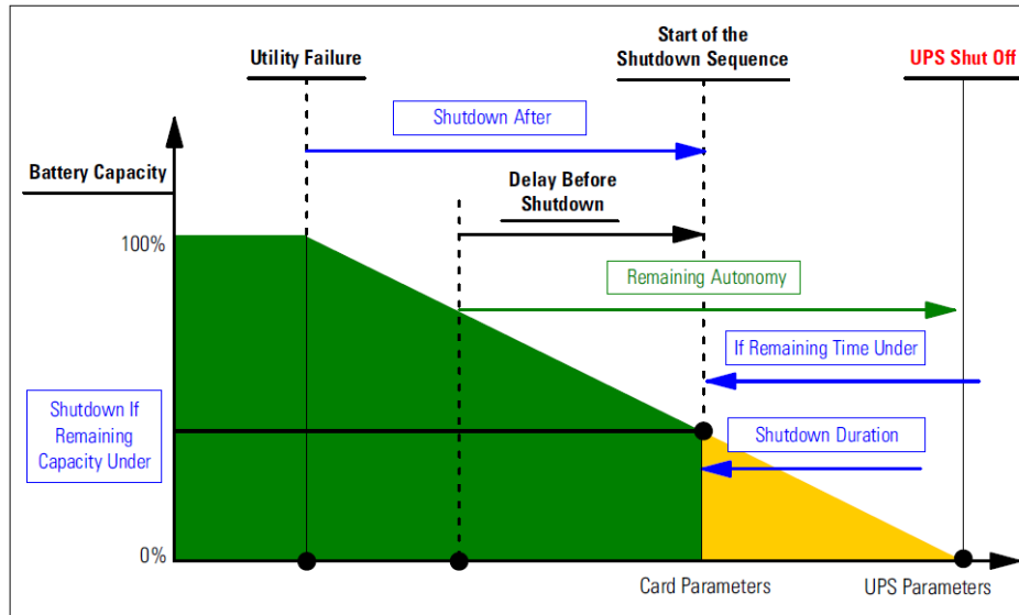
Shutdown Sequence Diagram
